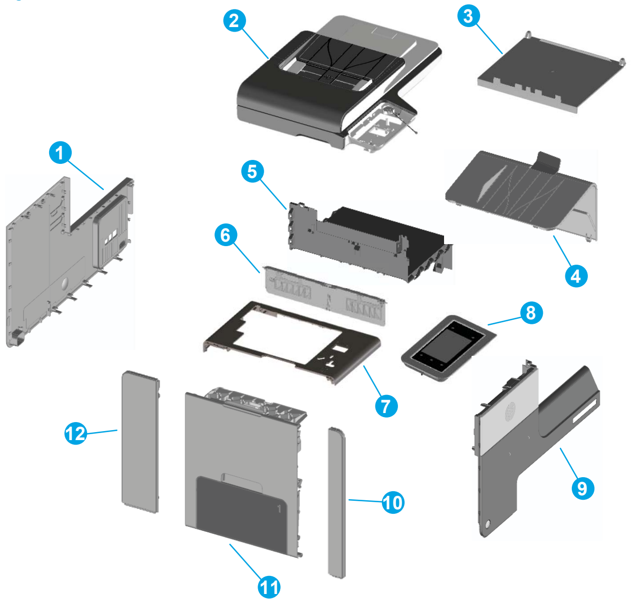
Figure 2-3 Covers (377/477 models)
